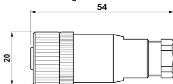
Dimensioned drawing
